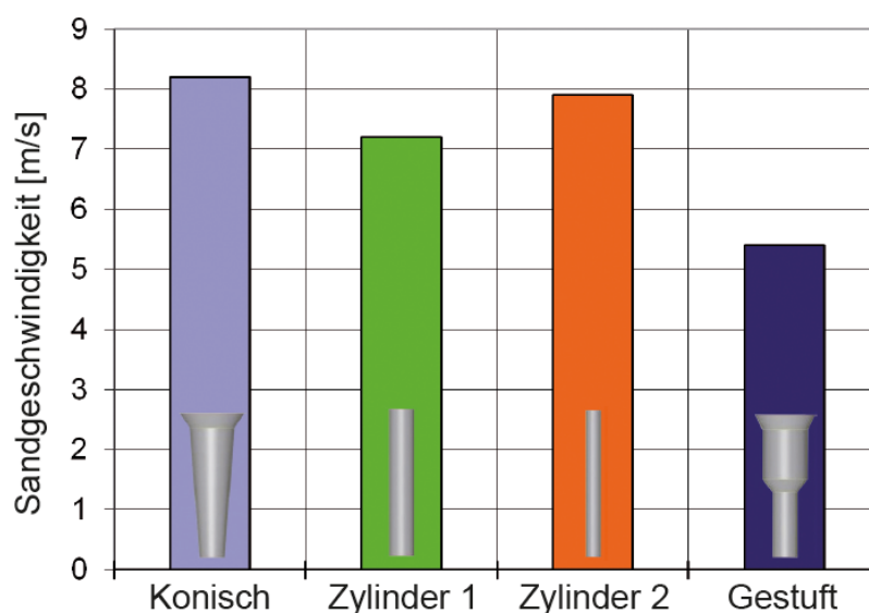
Figure 7: Measured velocities at exit of several different nozzles. The velocity is highly dependent on the nozzle geometry (at a given equal boundary condition). The same exit diameter of a cylindrical nozzle "Zylinder 1" and a stepped nozzle "Gestuft" lead to drastically different velocities.
