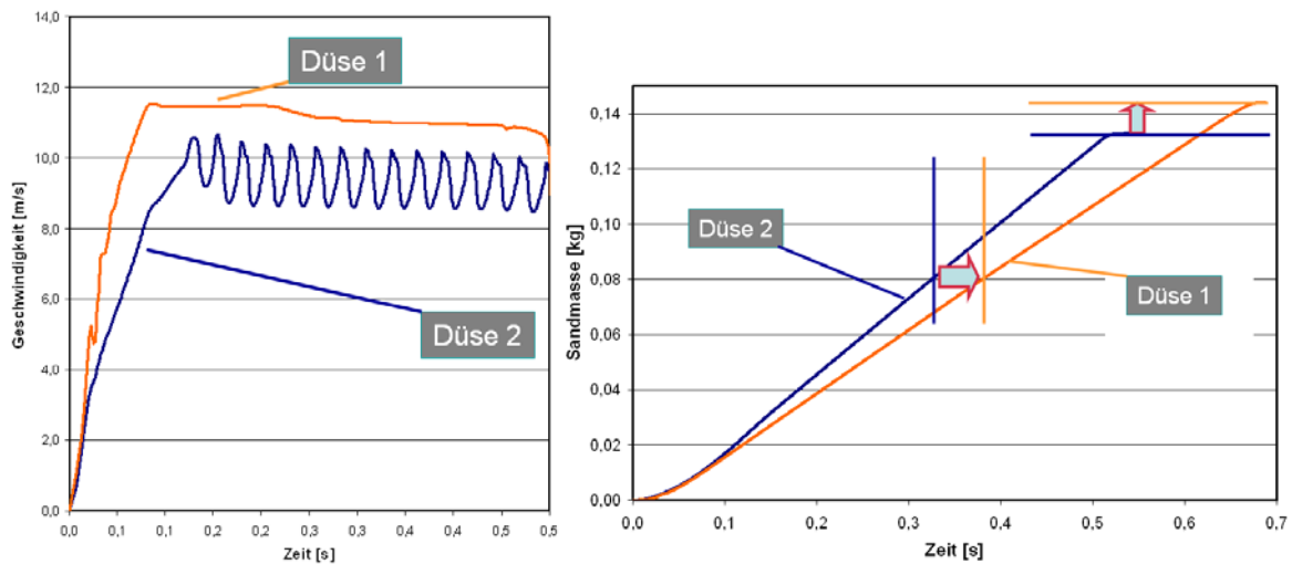
Figure 9: Sand velocities and amount of sand as function of time for two different nozzle geometries. The velocity (a) and the amount of sand as well differ for nozzles with equal nozzle diameter dependent on their geometry. The resulting sand amounts leads (dependent on the core geometry) to different compaction grades (b) . Here: "Düse 2" fills the corebox faster, but the total amount of sand is smaller. The core is, therefore, a little less compacted.
