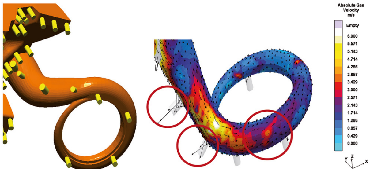
Figure 4: Configuration of vents in initial setup (a) and air velocity profile (b) .
