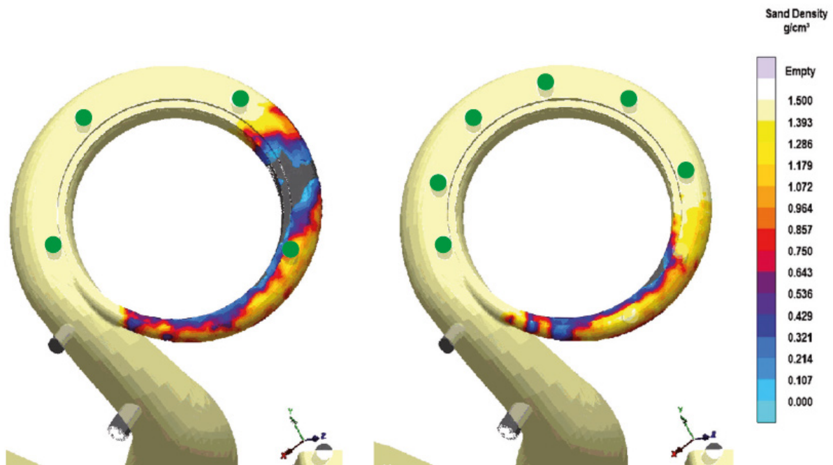
Figure 3: Simulated result for different vent configurations (a) 4 vents (b) 6 vents
