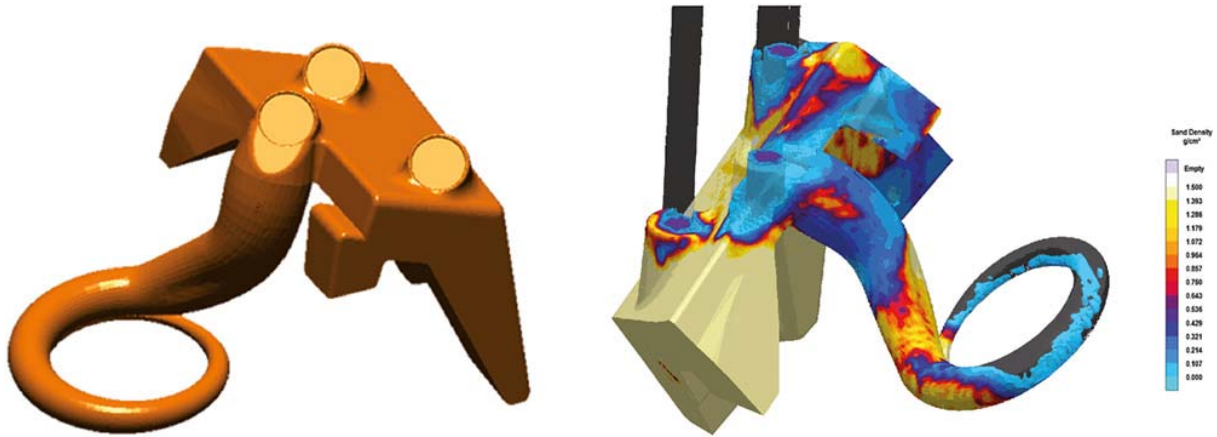
Figure 1: Turbocharger core geometry (a) and sand/binder mixture density distribution during the core shooting process (b).
