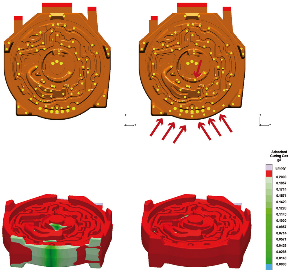
Figure 12: Comparison of gassing efficiency between the original (a) and the improved venting configuration (b) . The manipulation of the gas flow leads to the sufficient flooding of the entire core.
