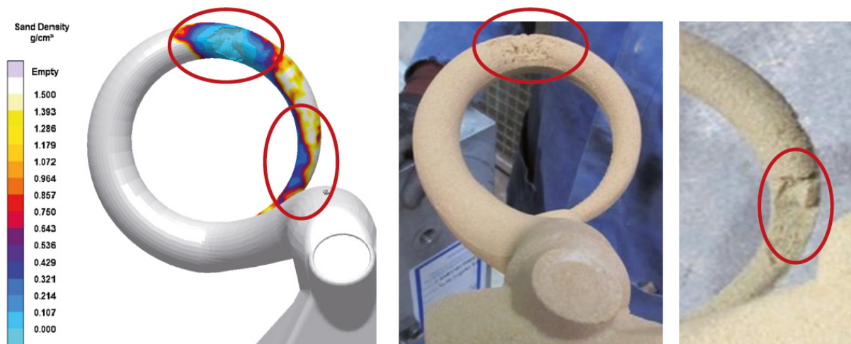
Figure 2: Predicted density distribution in the volute of the core (a) and real defects in prototype core of the initial corebox layout (b) and (c).
