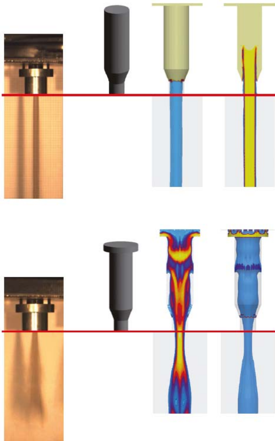
Figure 8: Comparison between real and simulated sand flows for different nozzle geometries. The sand typically flows as continuous stream out of the nozzle (a) . A geometrical change can change the sand flow into a discontinuous, pulsing flow (b) , where the stream widens. Depending on the core geometry, this can lead to a better core quality. Simulation permits for the differentiated evaluation of flow processes in nozzles (c) and (d) .
