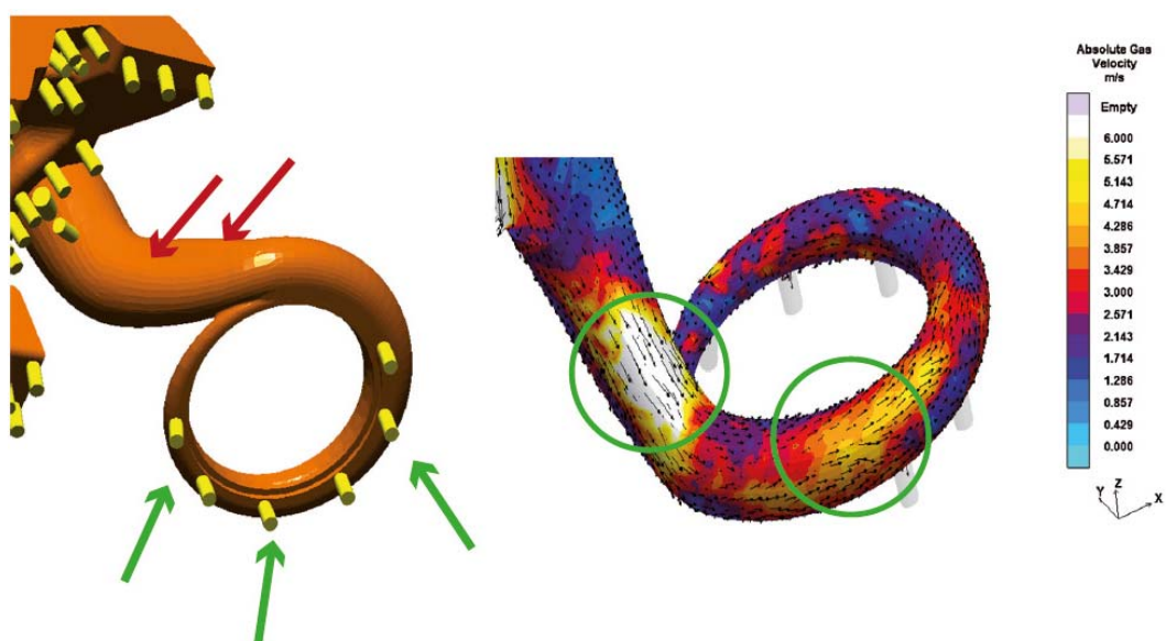
Figure 5: Vent configuration of optimized corebox (a) and improved flow profile of the air (b) .
