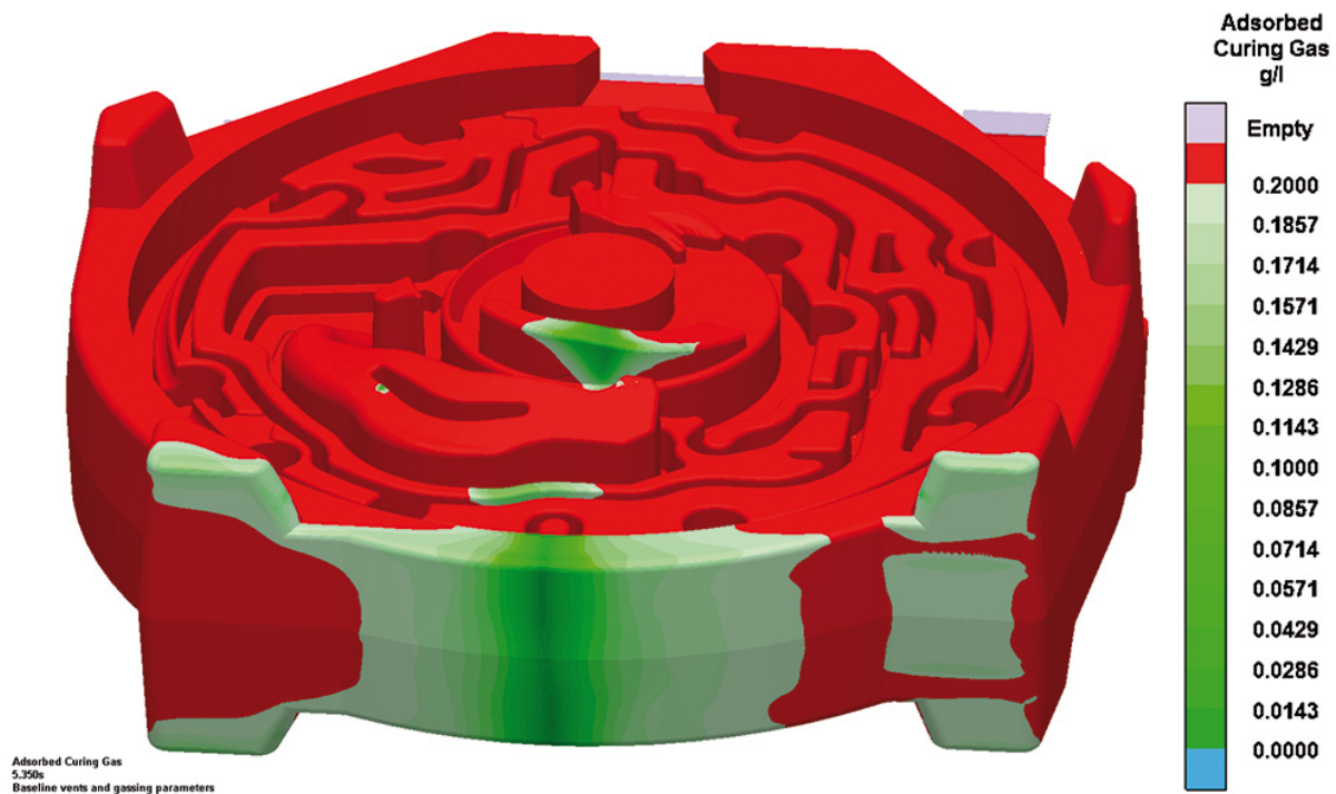
Figure 11: Amine gassing simulation. The concentration of absorbed amine is shown indicating the degree of curing. Completely cured areas are shown in red, incompletely cured areas in green (the darker the green, the less cured).
