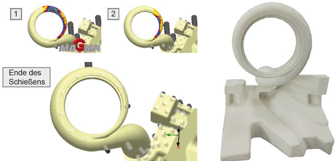
Figure 6: Compaction progress the volute at the end of the core shooting process (left) and optimally shot core (right).
